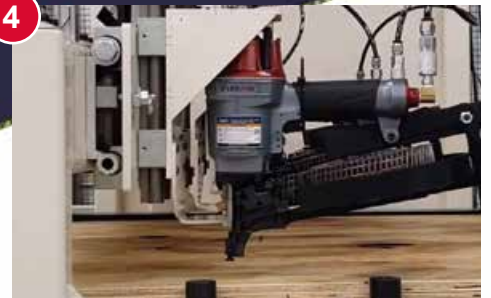
Automation: PN80PAL-JM at a sheathing station
