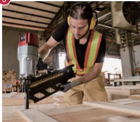
FSN160 securing deck boards to pallet jacks on a machinery crate
