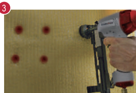
FS9240BC securing insulation layers
