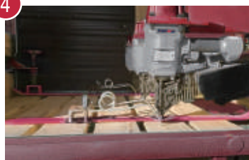
Automation: PN80PAL nailing decks to stringers
